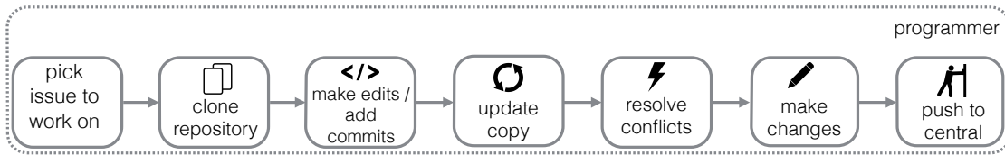
Fig. 2. Centralized workflow reported by one commercial team in our study, using Git commands instead of SVN.
